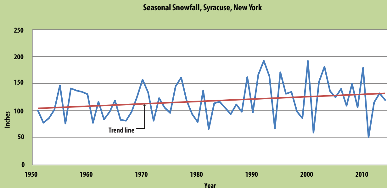
FIGURE 3- SEASONAL SNOWFALL IN SYRACUSE, NY, 1949-50 TO 2014-15 SOURCE: NATIONAL WEATHER SERVICE FORECAST OFFICE
